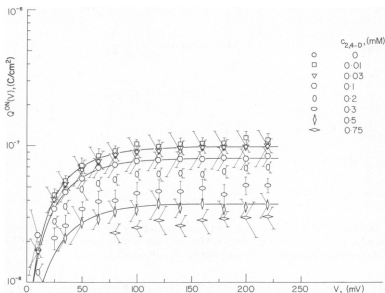
FIGURE 4 The effect of 2,4-D on the transfer of electric charge associated with \text{TPhB}^- ions across PC-chol membranes. The solid curves have been drawn according to Eq. 5 for \beta = 0.91 .
