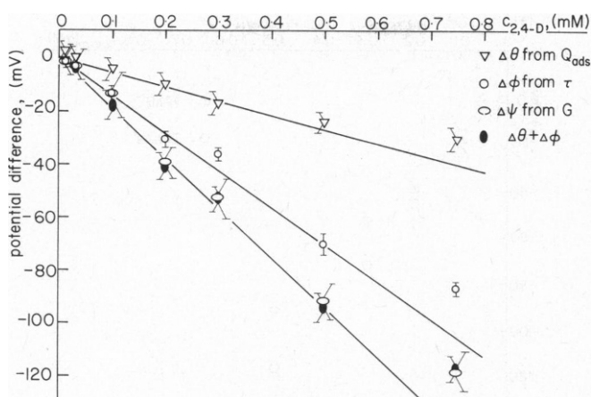
FIGURE 7 Changes of various electric potential differences as a function of aqueous 2,4-D concentration determined from the studies of relaxation of \text{TPhB}^- conduction current in PC-chole membranes. \Delta\theta is the change of the potential difference between the \text{TPhB}^- adsorption plane and the aqueous solution, \Delta\phi is the change of the potential difference between the central membrane plane and the adsorption plane. \Delta\psi is the change of the potential difference between the central membrane plane and the aqueous solution.
